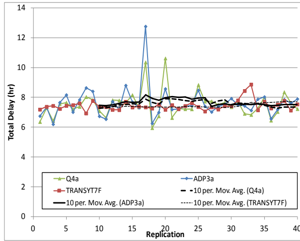
19b – Total vehicle delay
