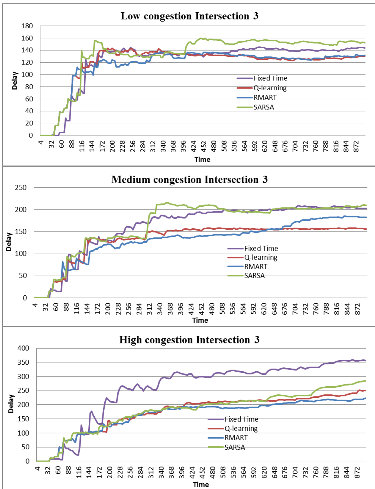
Figure 5 Comparison of algorithms (Reward-1).
